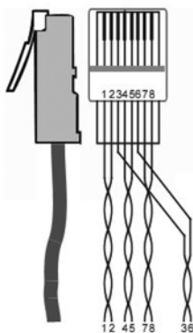
Cable pinout diagram.
